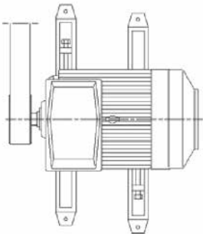
Figure 2. Belt drive
